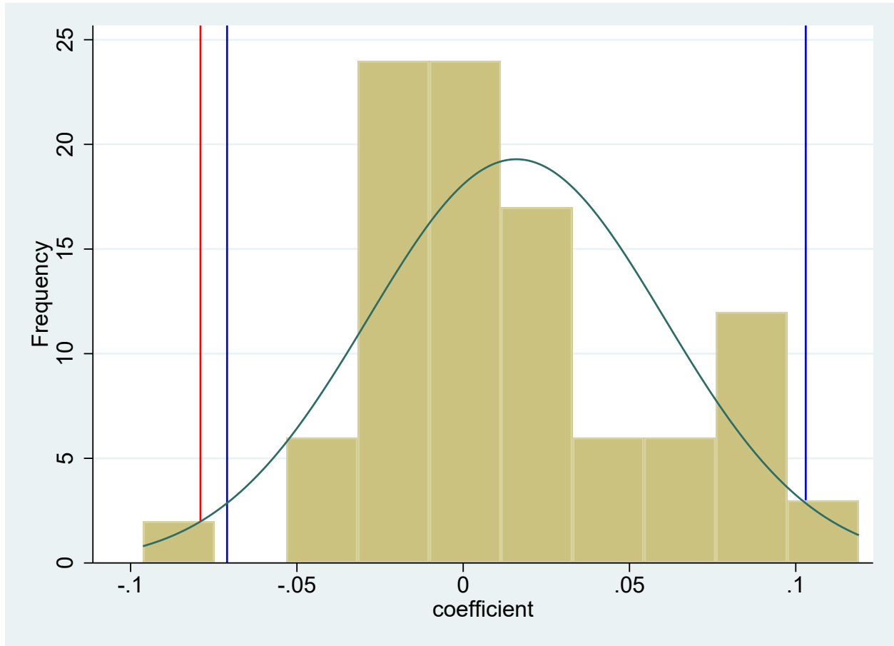
Figure A.1: The figure plots the coefficients from 100 iterations of running the RD Equation 3, with random cut-offs. The bandwidth is set at 0.1 in each iteration. The blue lines show the 95th percentile of the distribution on either side of the mean, while the red line shows our main RD coefficient with cut-off set at zero.
