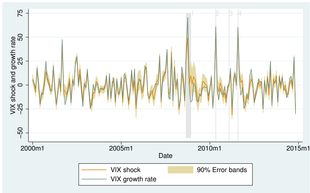
Figure 1: The estimated US uncertainty shock and the growth rate of VIX
